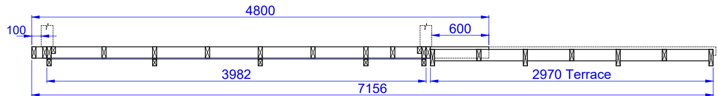
Cut view
