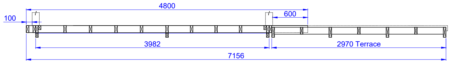
Cut view
