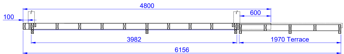
Cut view
