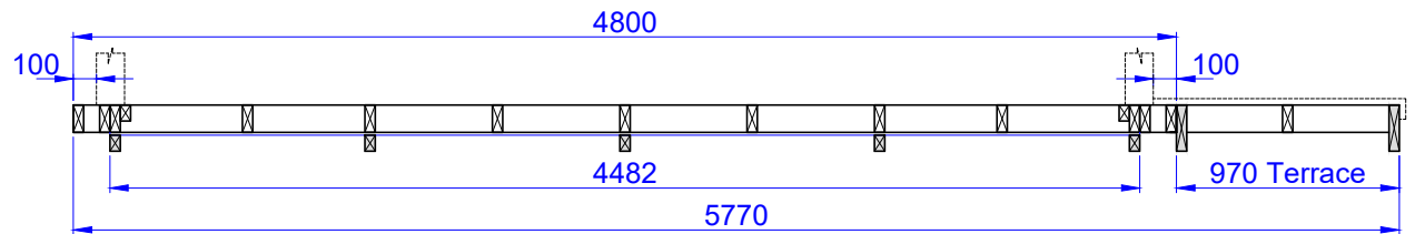
Cut view
