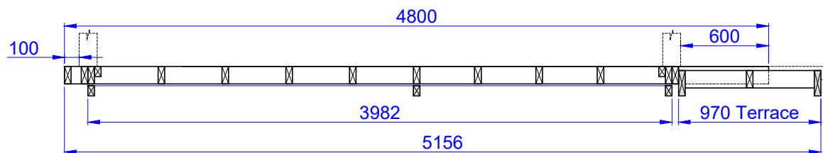
Cut view
