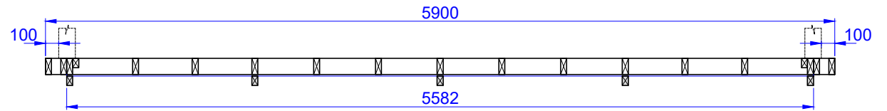
Cut view
