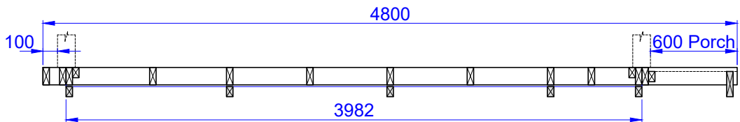
Cut view
