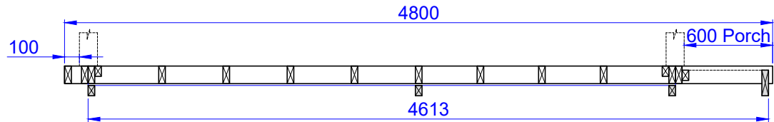
Cut view
